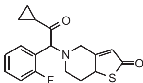
Prasugrel Desacetyl Impurity
