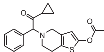
Prasugrel Desfluoro Impurity
