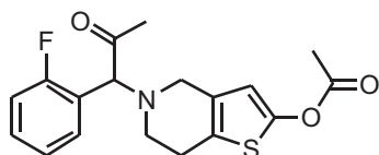
Prasugrel Acetyl Impurity
