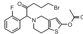
Prasugrel Bromobutyryl Impurity
