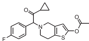
Prasugrel 4-Fluoro Impurity
