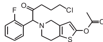
Prasugrel Chlorobutyryl Impurity
